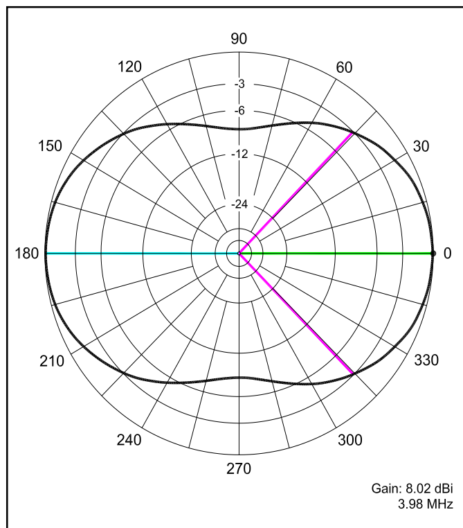
Figure 2—Azimuth pattern at an elevation of 30 degrees for the antenna of Figure 1.
